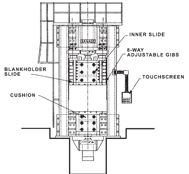
Slide within blankholder
