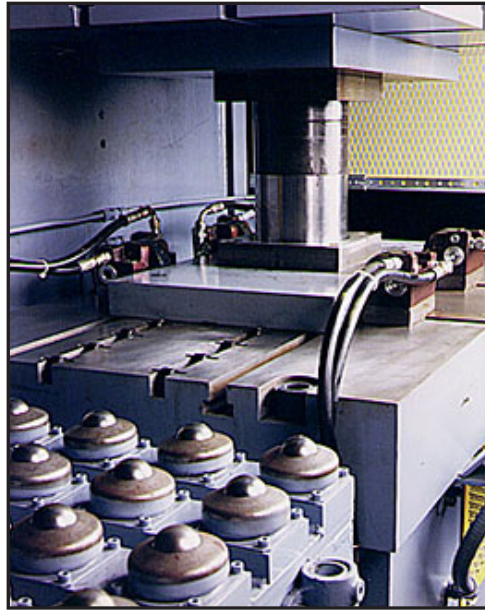
Die staging table and hydraulic clamps
