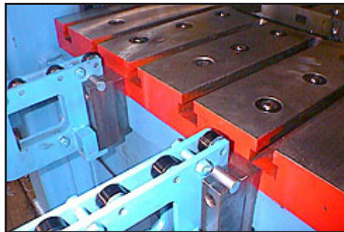
Slug Chute - Die Locators Die Rollers - Ext. Rails
