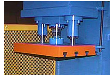
2 post/4 Bushing Guided Platen
