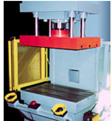
4 post/8 Bushing Guide System
